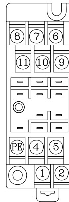
Pin Location
