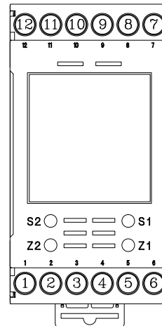
Pin Location
